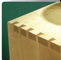
Through Dovetails
