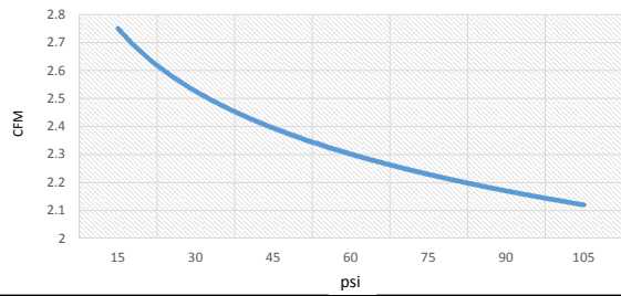
Swan DRS-210-30 Free Air Delivery
