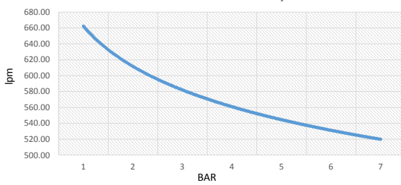
Swan SVP205 Free Air Delivery
