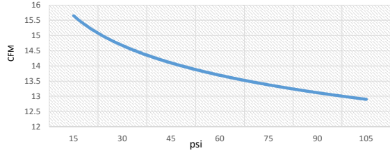
Swan SVP205 Free Air Delivery
