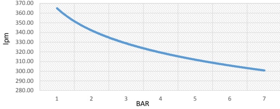
Swan SVP205 Free Air Delivery
